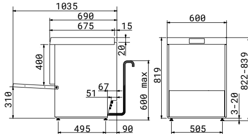
Raised Traywasher 500×500
