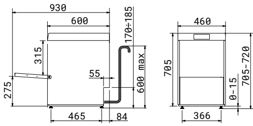
Undercounter Dishwasher 500×500
