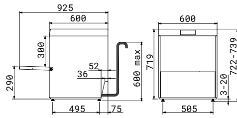
Undercounter Traywasher 500×500
